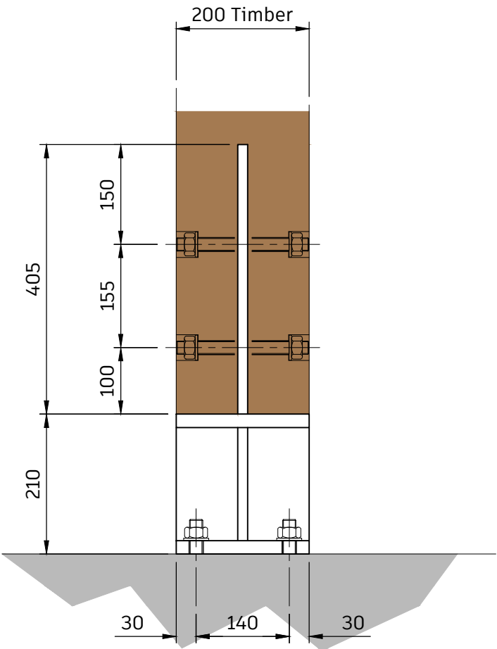
Front Elevation (NTS)
